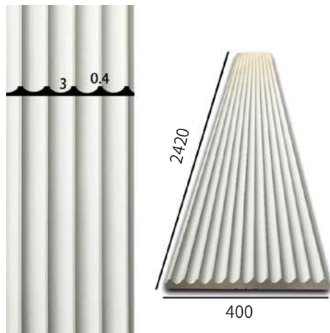
SCTP28 Size: 2420x400mm
