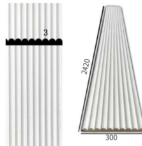
SCTP26 Size: 2420x300mm
