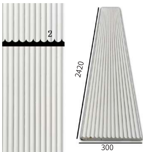
SCTP23 Size: 2420x300mm
