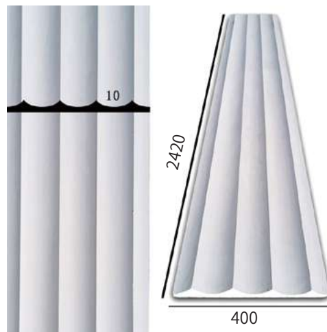
SCTPA32 Size: 2420x400mm
